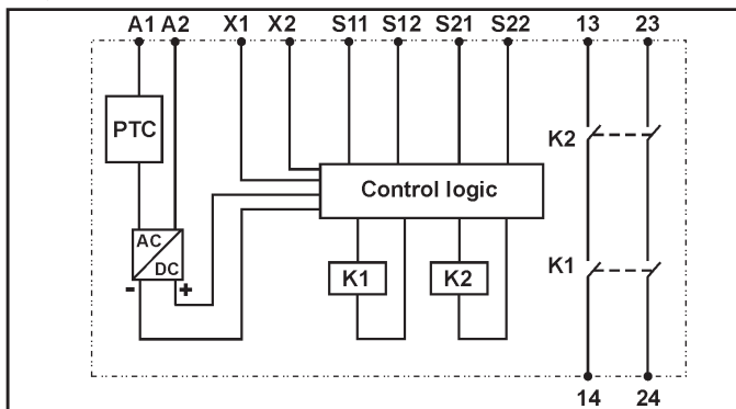
Fig. 1 - NA1/2-D diagram
