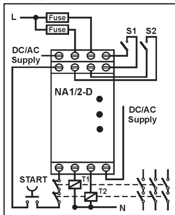
Fig. 2: NA1/2-D application
